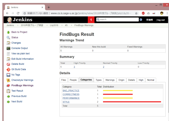
Figure 2: Result of static code checking.
