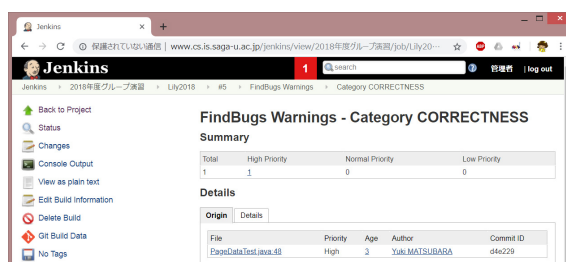
Figure 3: FindBugs warnings belonging to the CORECTNESS category.
