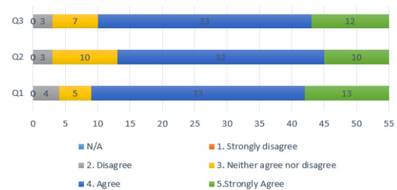
Figure 9: Evaluation of ALECSS at week 15.
